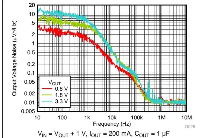
Figure 45. Output Noise vs Frequency and V_{OUT}
