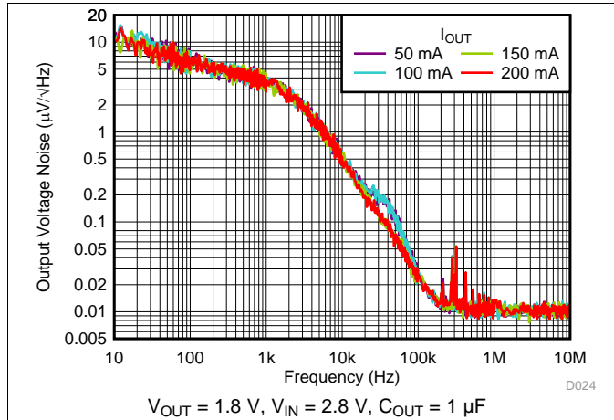
Figure 43. Output Noise vs Frequency and I_{OUT}
