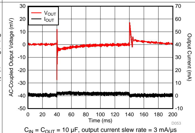
Figure 16. I_{OUT} Transient 3 \mu\text{A} to 3 mA
